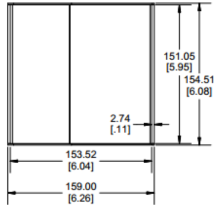
TOP VIEW OF ENCLOSURE
