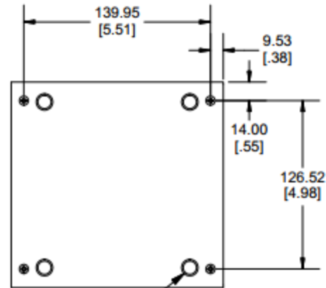
BOTTOM VIEW OF ENCLOSURE
