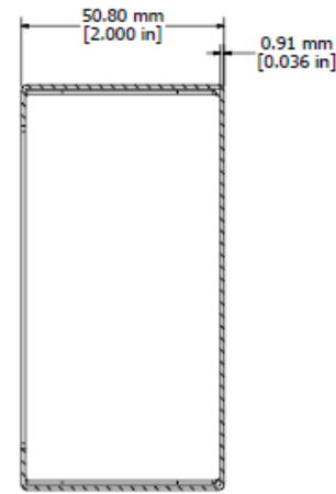
SECTION EE-EE
